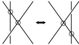
FIGURE 1.6. The mixed Reidemeister move
